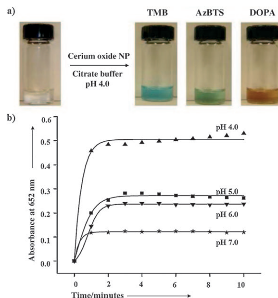
Figure 1. Formation of colored product owing to substrate oxidation is pH-dependent. a) Photographs show production of colored product upon addition of nanoceria to TMB, AzBTS, and DOPA at pH 4.0. b) Oxidation of TMB is pH-dependent, with the optimum activity at pH 4.0.
