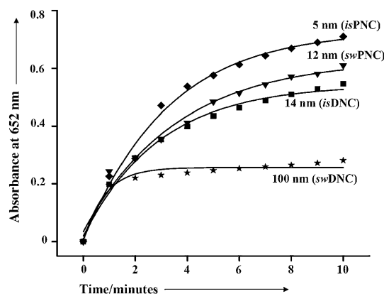
Figure 2. Nanoceria-promoted oxidation of TMB is size-dependent. At pH 4.0, smaller ceria nanoparticles show higher oxidase-like activity than larger nanoparticles.
